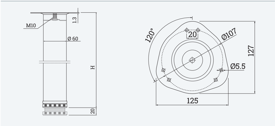
Technical Drawing
