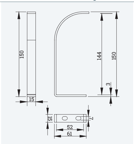
Technical drawings
