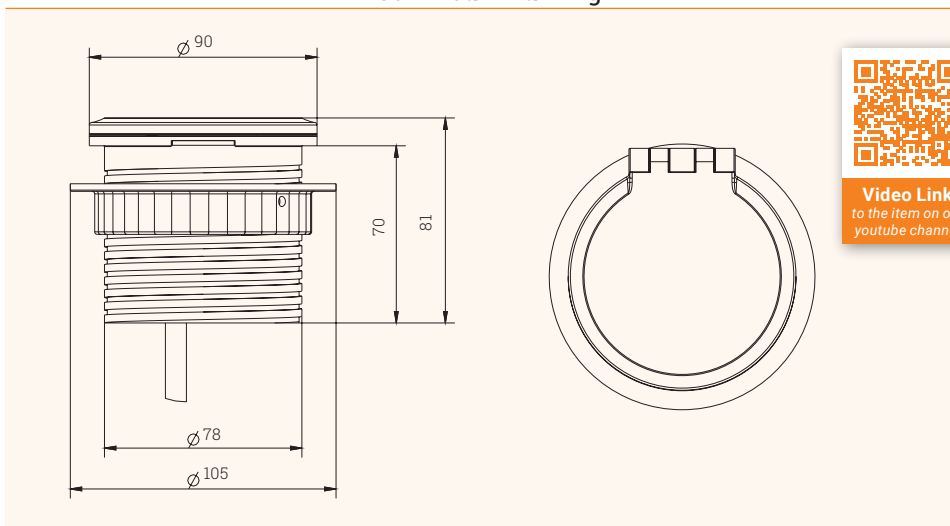
Technical Drawing
