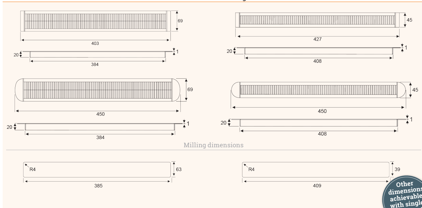
Technical Drawings
